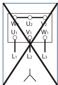
3 Incorrect connection
